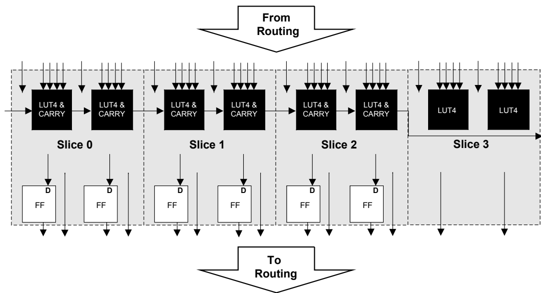
Figure 2-2. PFU Diagram
