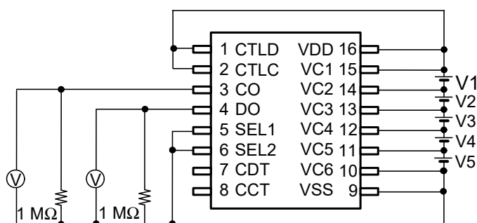
Figure 7 Test Circuit 4
