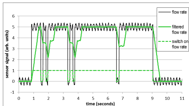
Figure 3: Cable output with moving average filter on flow rate (green solid line) and switch output on unfiltered flow rate (green dashed line). The black line shows the underlying unfiltered flow rate.
