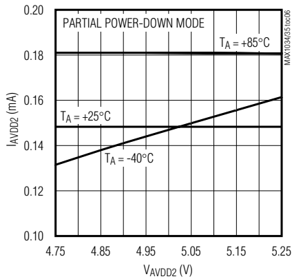
PREAMPLIFIER SUPPLY CURRENT vs. PREAMPLIFIER SUPPLY VOLTAGE
