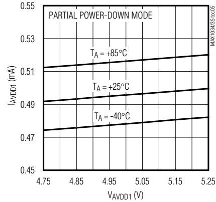
ANALOG SUPPLY CURRENT vs. ANALOG SUPPLY VOLTAGE
