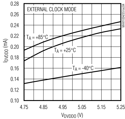
DIGITAL I/O SUPPLY CURRENT vs. DIGITAL I/O SUPPLY VOLTAGE
