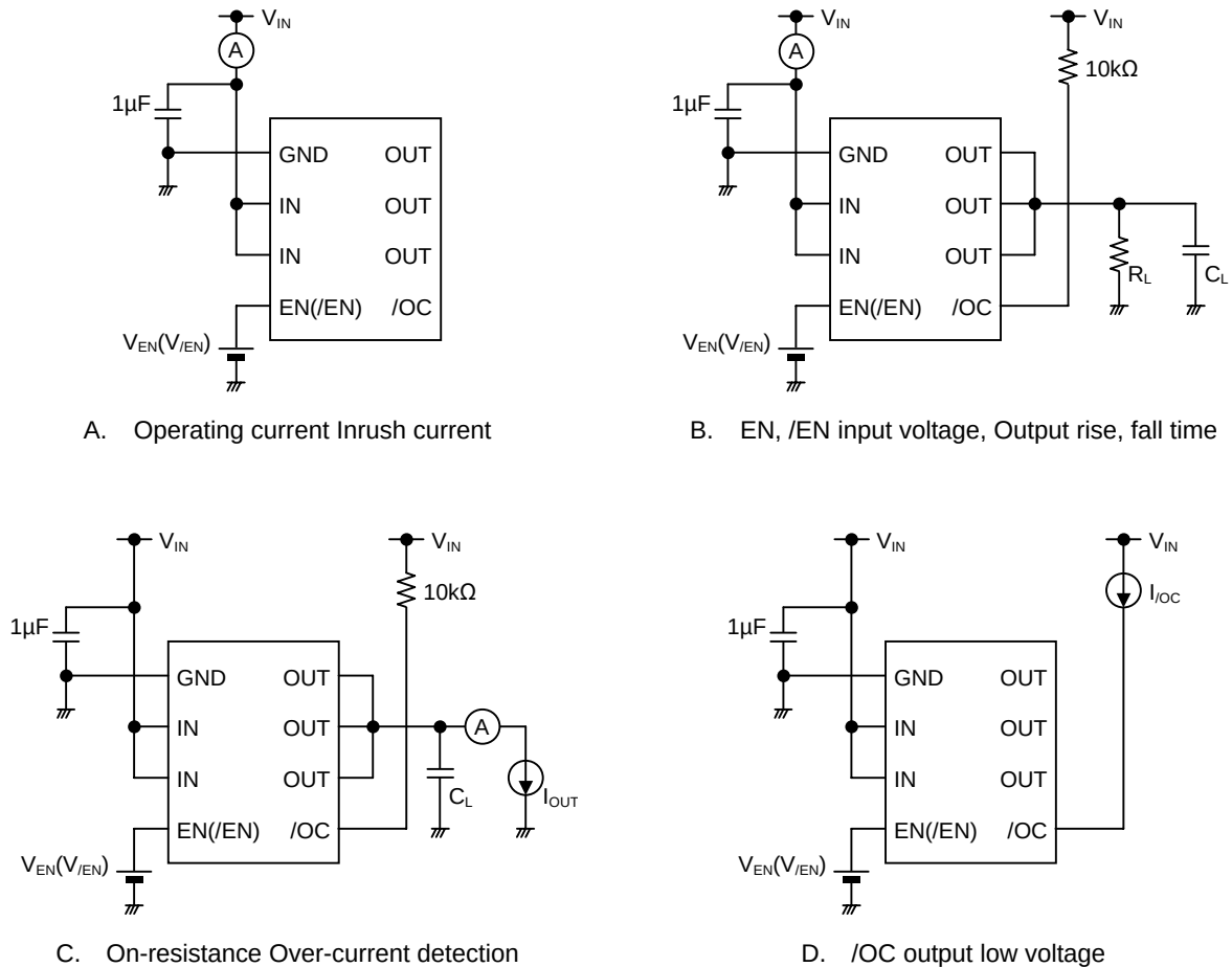
Figure 1. Measurement circuit
