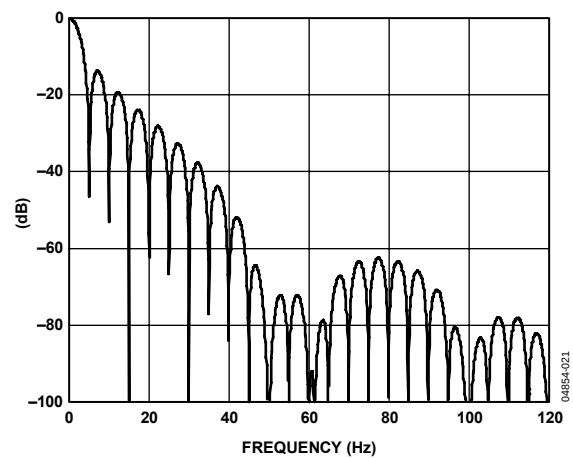
Figure 17. Filter Response with Update Rate = 4.17 Hz (Chop Disabled)
