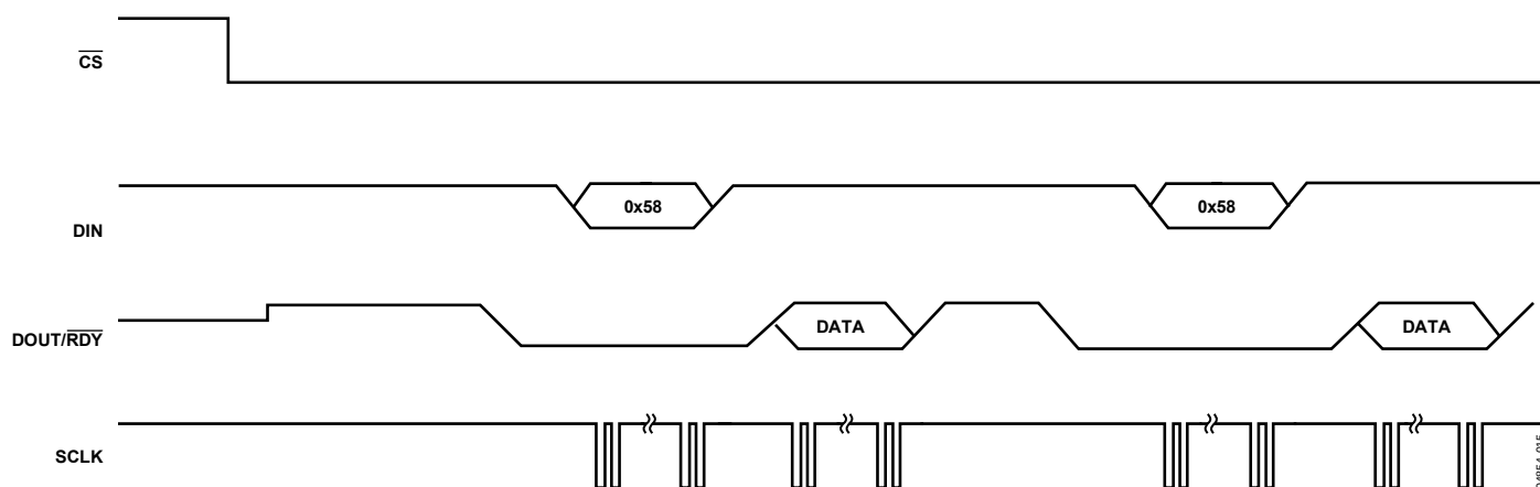
Figure 22. Continuous Conversion
