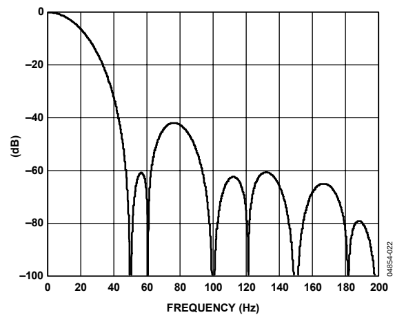
Figure 18. Filter Response with Update Rate = 16.7 Hz (Chop Disabled)
