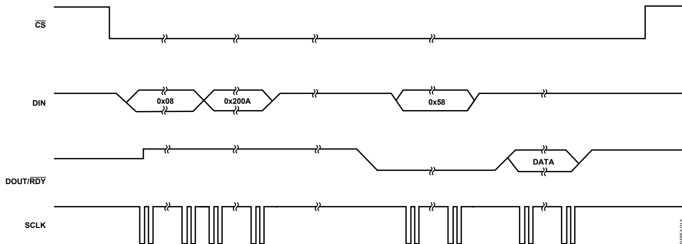
Figure 21. Single Conversion
