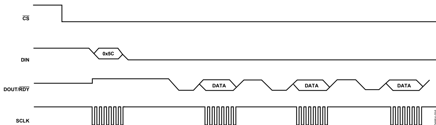
Figure 23. Continuous Read
