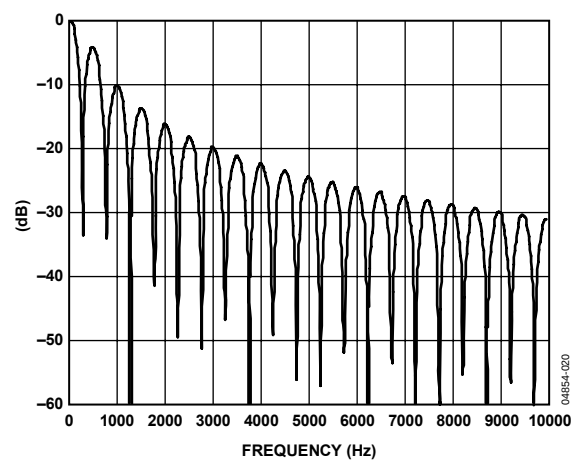
Figure 16. Filter Response with Update Rate = 470 Hz (Chop Enabled)
