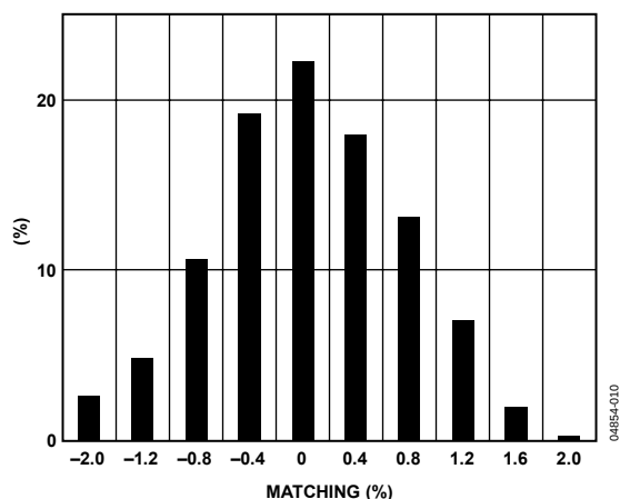
Figure 10. Excitation Current Matching (210 \mu A) at Ambient Temperature
