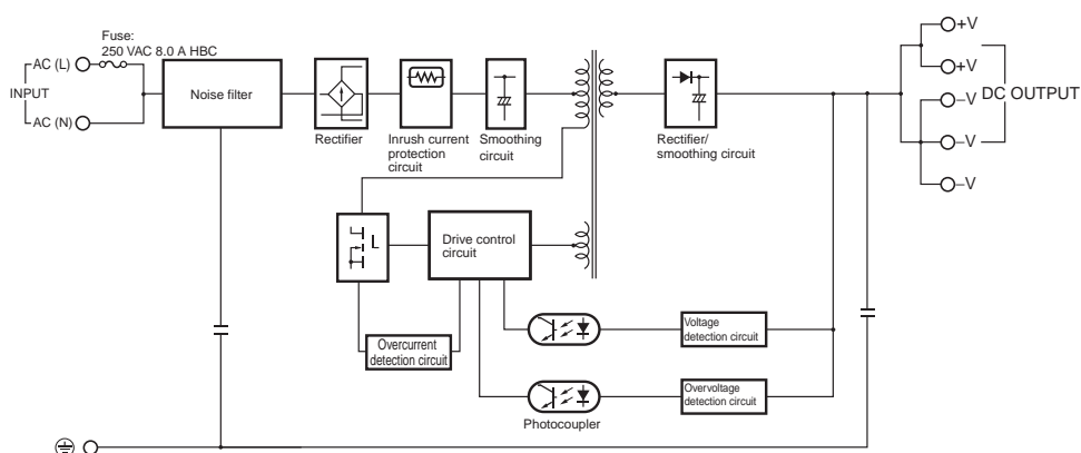
S8VK-C12024 (120W)
