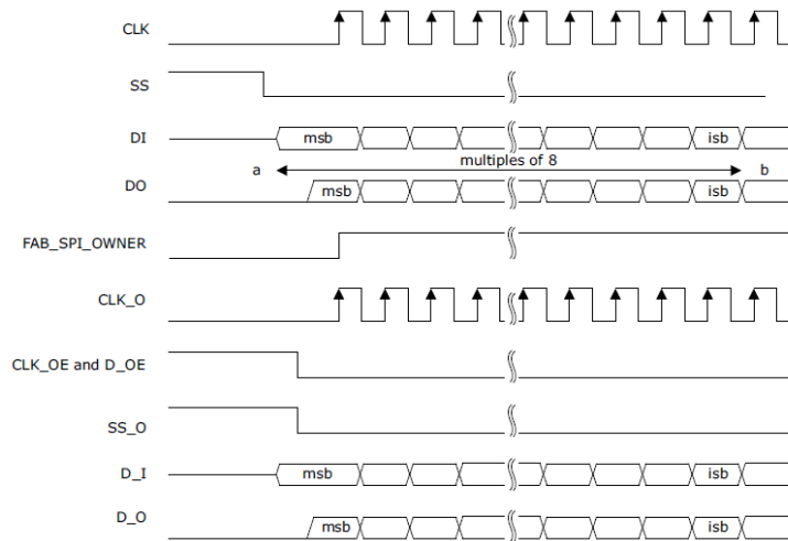
Figure 7 • USPI Switching Characteristics
