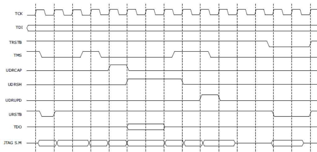
Figure 6 • UJTAG Timing Diagram
