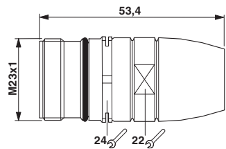
Dimensional drawing
