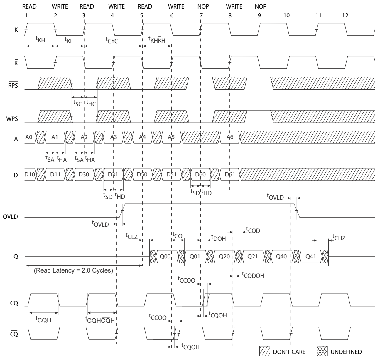
Figure 5. Waveform for 2.0 Cycle Read Latency [35, 36, 37]
