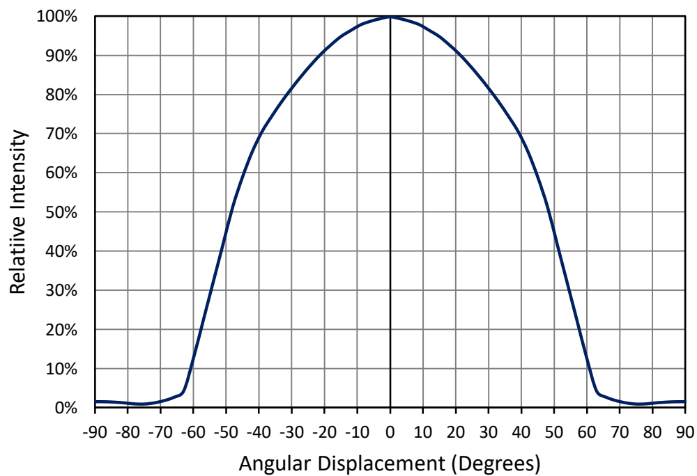
Figure 4: Typical representative spatial radiation pattern.
