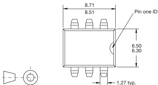
SMD
