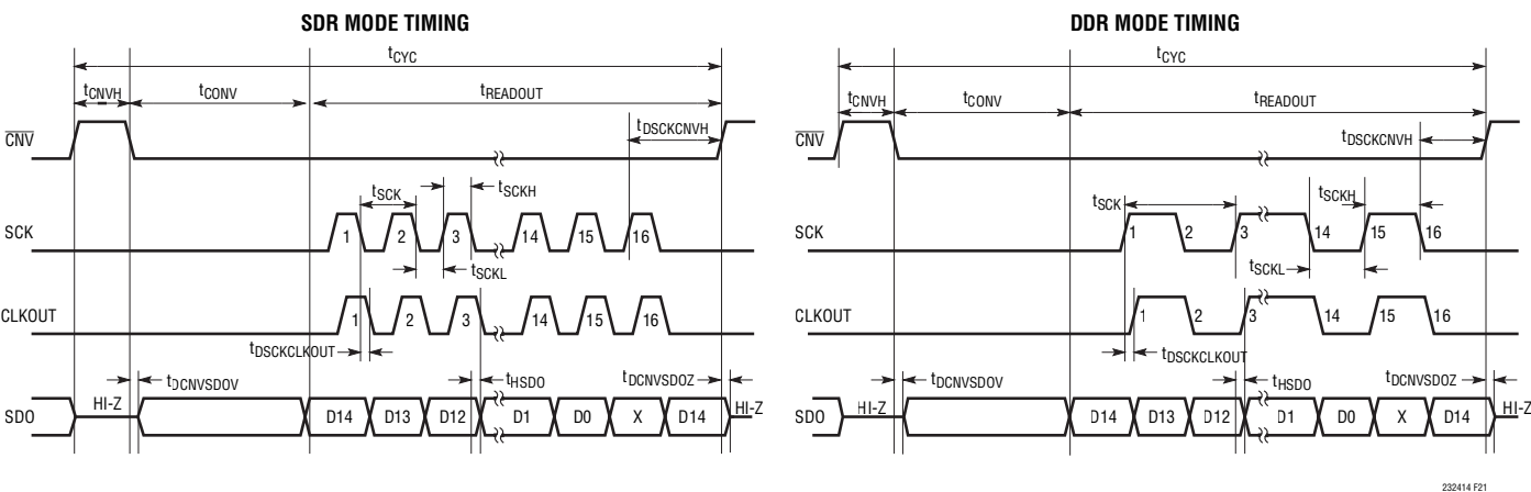
Figure 21. LTC2324-14 Timing Diagram
