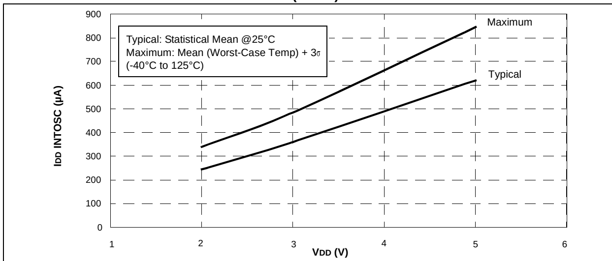
FIGURE 16-6: PIC16F610/616 I_{DD} INTOSC (4 MHz) vs. V_{DD}
