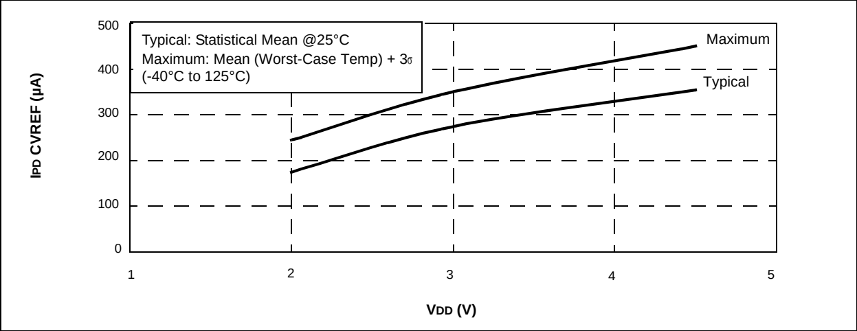
FIGURE 16-32: PIC16HV610/616 I PD CVREF (LOW RANGE) vs. V DD
