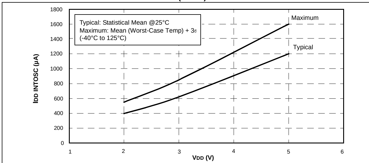
FIGURE 16-7: PIC16F610/616 I_{DD} INTOSC (8 MHz) vs. V_{DD}
