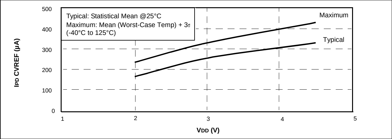
FIGURE 16-33: PIC16HV610/616 I PD CVREF (HI RANGE) vs. V DD
