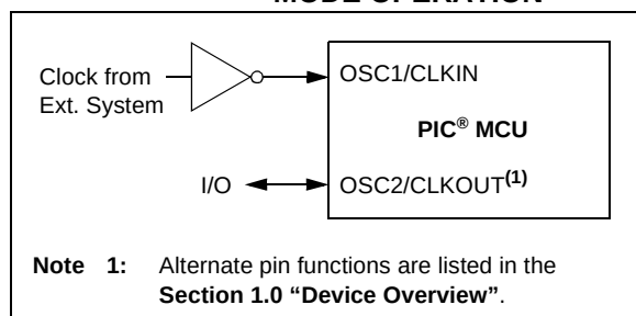
FIGURE 3-2: EXTERNAL CLOCK (EC) MODE OPERATION
