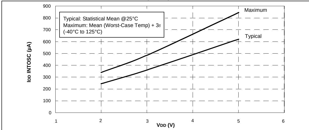
FIGURE 16-6: PIC16F610/616 I_{DD} INTOSC (4 MHz) vs. V_{DD}
