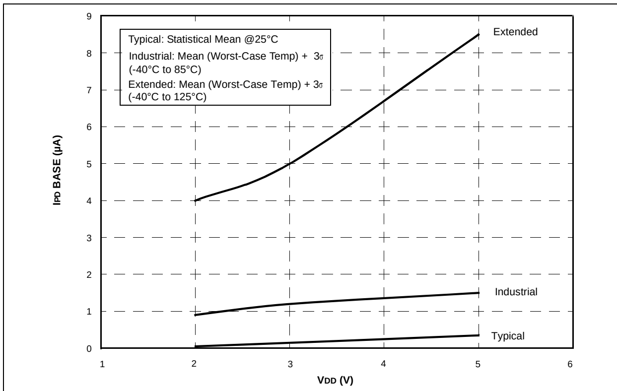
FIGURE 16-10: PIC16F610/616 I PD BASE vs. V DD
