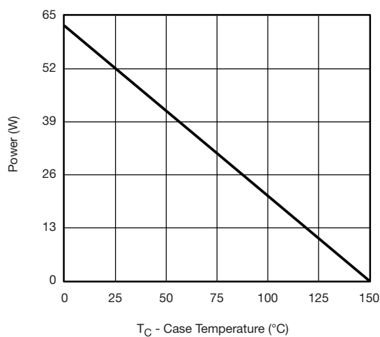
Power, Junction-to-Case
