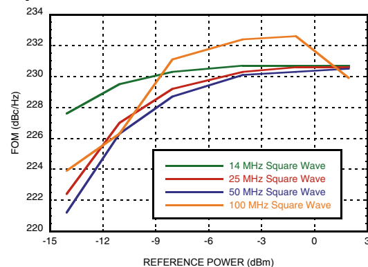
Figure 12. Reference Input Sensitivity, Square Wave, 50 \Omega [2]
