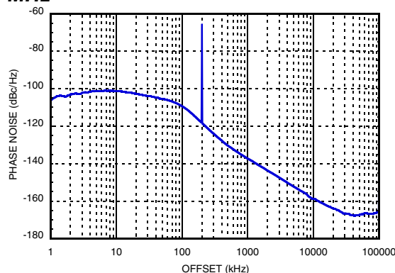
Figure 14. Integer Boundary Spur at 2500.2 MHz [4]
