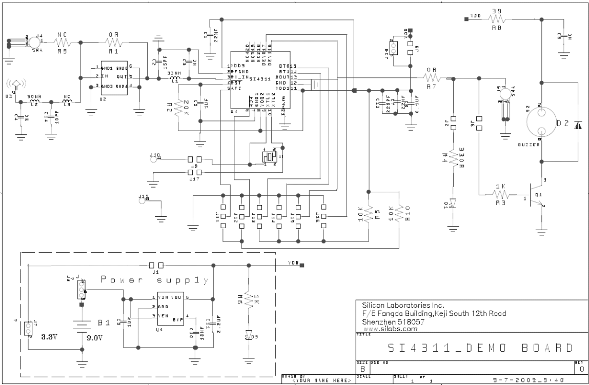
Figure 3. Si4311-DEMO Schematic
