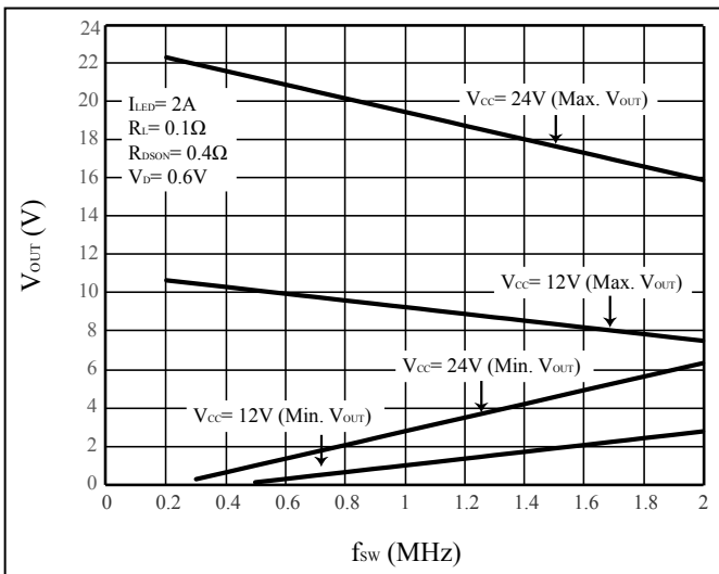
Figure 32 Minimum and Maximum Output Voltage versus Operating Frequency (minimum t_{ON} and t_{OFF} = 150ns )
