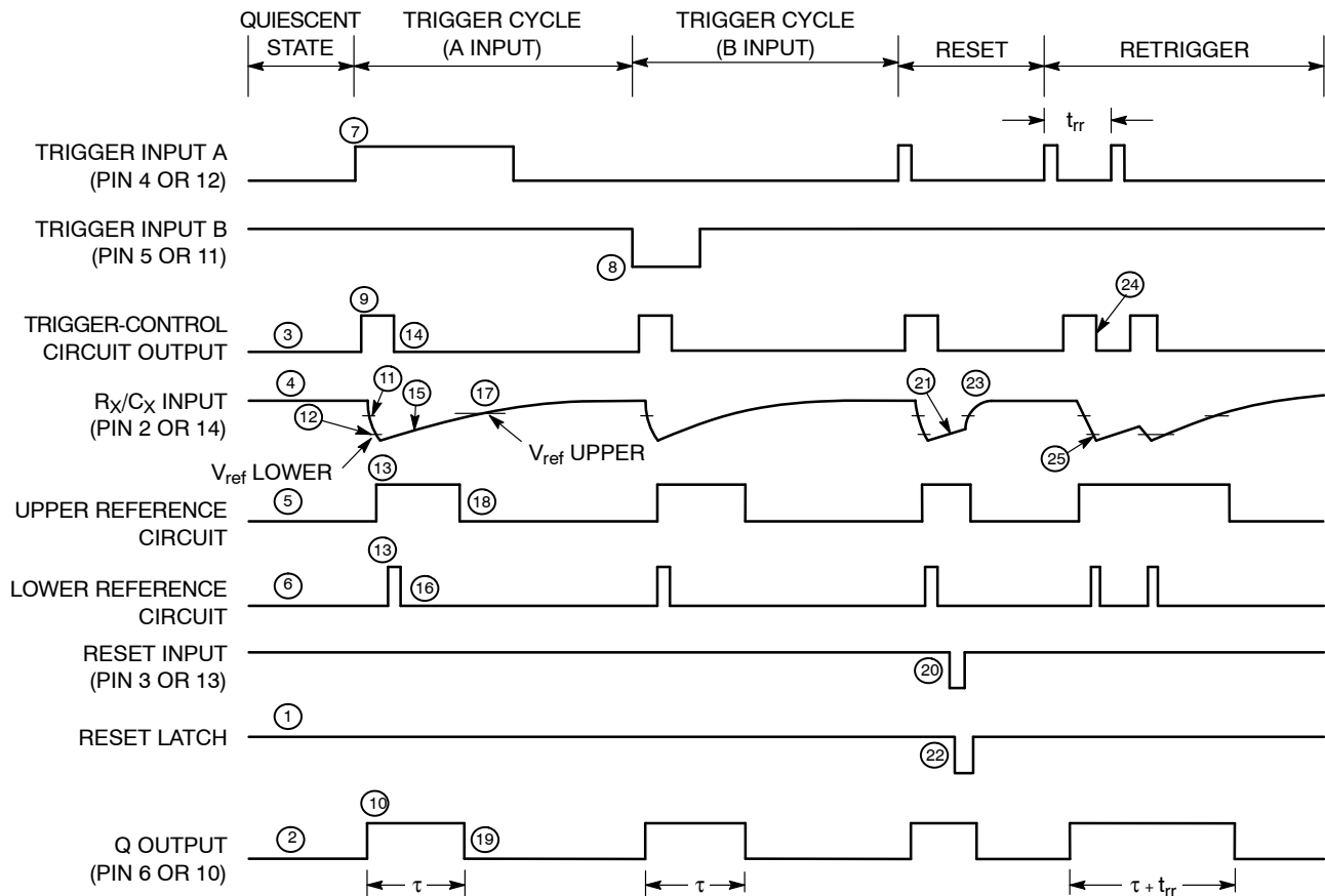
Figure 12. Timing Diagram
