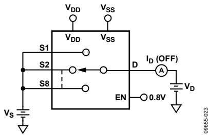
Figure 20. I_D (Off)
