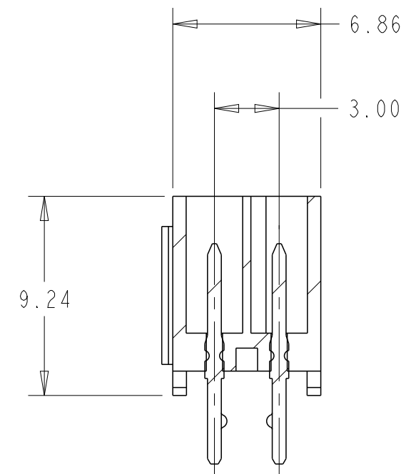
SECTION Z-Z
