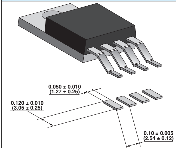
FIGURE 8 - VPR221S LAND PATTERN DIMENSIONS in inches (millimeters)
