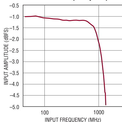
LTC2155-12: Frequency Response
