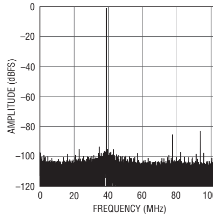
LTC2156-12: 32K Point FFT, f_{IN} = 171\text{MHz} , -1dBFS, 210Mps
