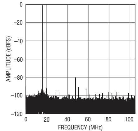
LTC2156-12: 32K Point FFT, f_{IN} = 227\text{MHz} , -1dBFS, 210Mps
