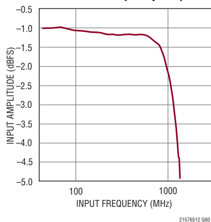
LTC2155-12: Frequency Response
