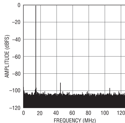
LTC2157-12: 32K Point FFT, f_{IN} = 15\text{MHz} , -1\text{dBFS} , 250Msps
