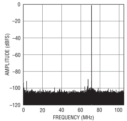
LTC2156-12: 32K Point FFT, f_{IN} = 71\text{MHz} , -1dBFS, 210Mps
