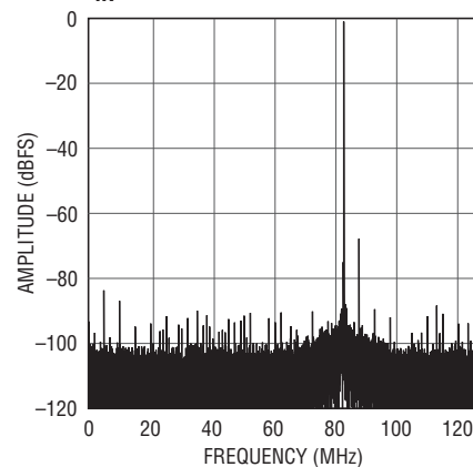
LTC2157-12: 32K Point FFT, f_{IN} = 420\text{MHz} , -1\text{dBFS} , 250MHz
