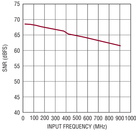
LTC2157-12: SNR vs Input Frequency, -1dBFS, 1.5V Range, 250Mps
