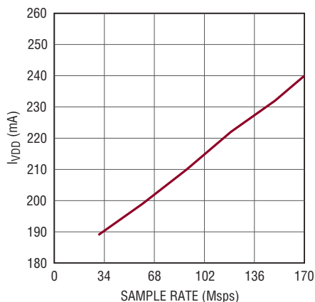
LTC2155-12: I_{VDD} vs Sample Rate, 15MHz Sine Wave Input, -1dBFS
