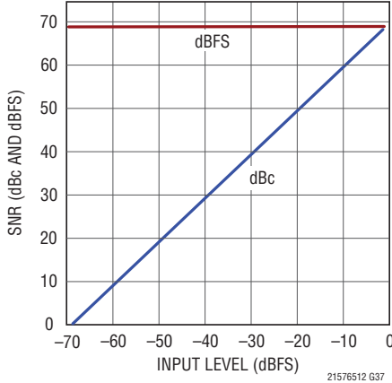
LTC2156-12: SNR vs Input Level, f_{IN} = 70\text{MHz} , 1.5V Range, 210Mps
