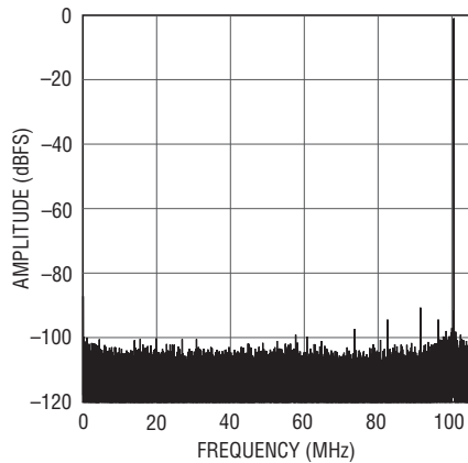
LTC2156-12: 32K Point FFT, f_{IN} = 101\text{MHz} , -1dBFS, 210Mps
