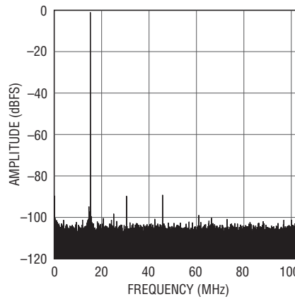
LTC2156-12: 32K Point FFT, f_{IN} = 15\text{MHz} , -1dBFS, 210Mps
