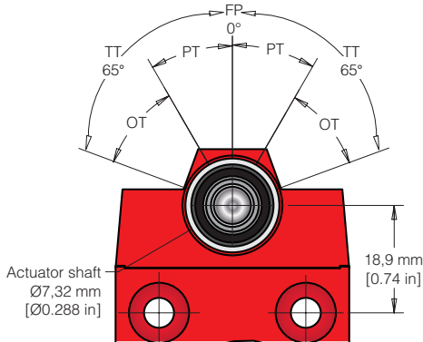
Figure 6. 924CE16 Dimensions
