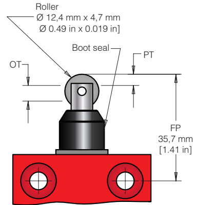
Figure 11. 924CE31 Dimensions
