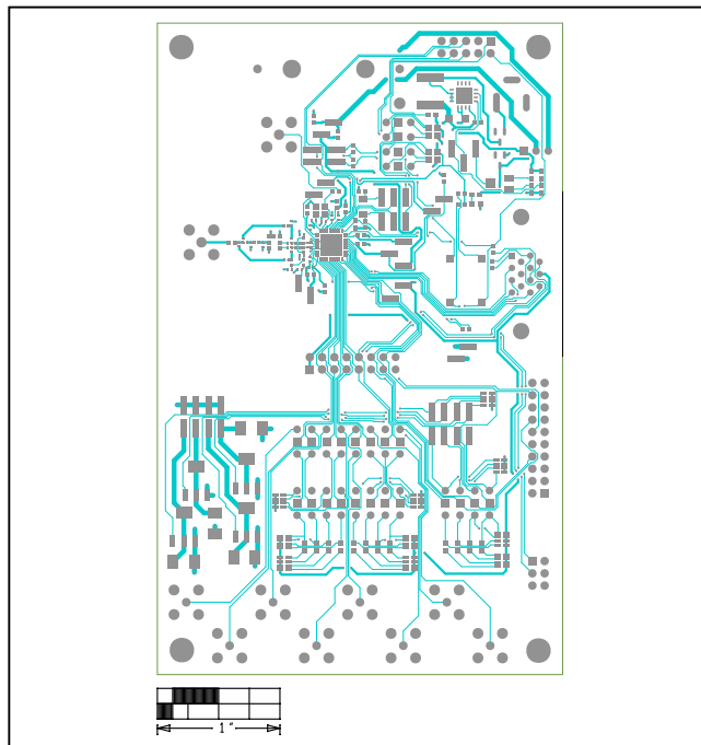
MAX7037 EV Kit—Top
