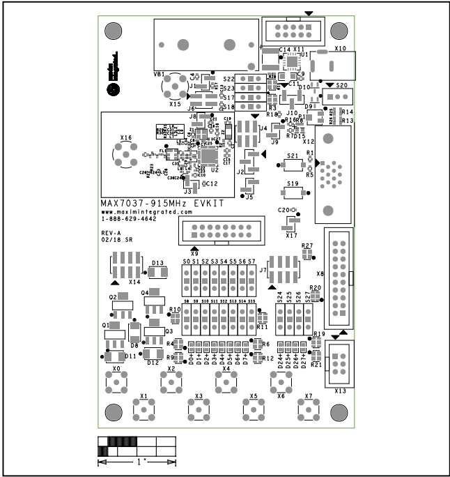
MAX7037 EV Kit—Top Silkscreen
