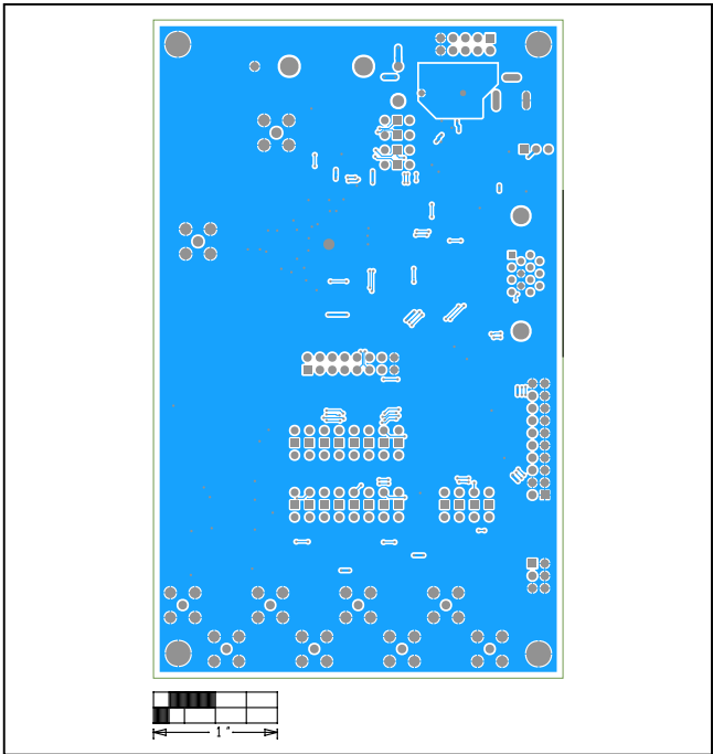
MAX7037 EV Kit—Bottom
