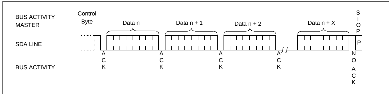
FIGURE 8-3: SEQUENTIAL READ
