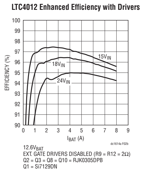
Figure 2. Efficiency Comparison with and without External Gate Drivers at 15V IN , 18V IN , and 24V IN
