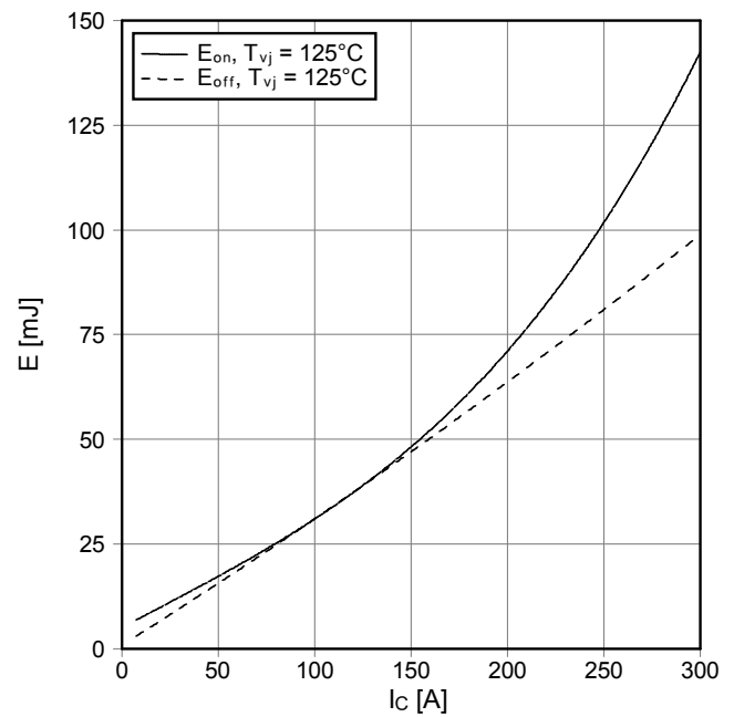
Schaltverluste IGBT-Wechselr. (typisch) switching losses IGBT-inverter (typical) E_{on} = f(I_c), E_{off} = f(I_c) V_{GE} = \pm 15\text{ V}, R_{Gon} = 9.1\ \Omega, R_{Goff} = 9.1\ \Omega, V_{CE} = 900\text{ V}
