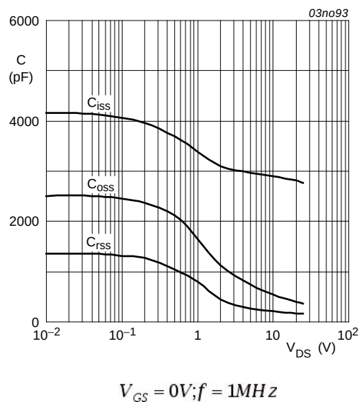
Fig 14. Input and reverse transfer capacitances as a function of gate-source voltage; typical values
