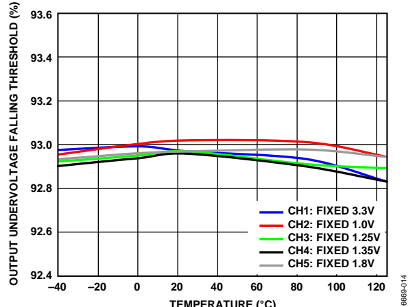
Figure 14. Output Undervoltage Falling Threshold vs. Temperature
