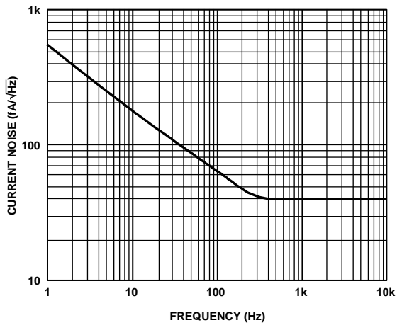
Figure 30. Current Noise Spectral Density vs. Frequency
