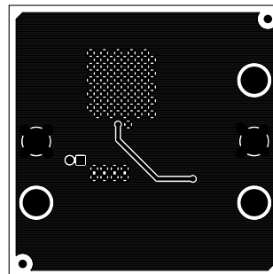
Solder Side
