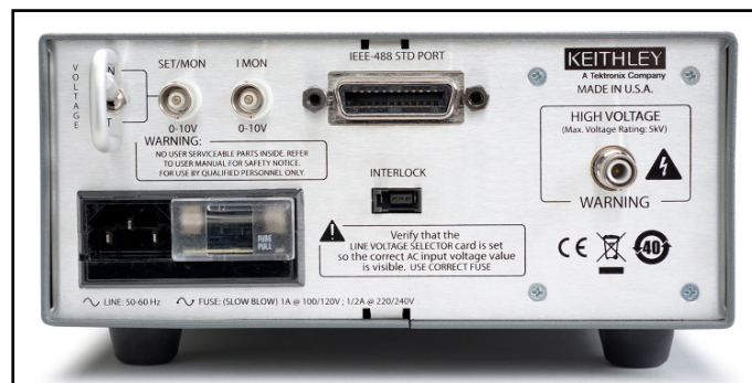
Model 2290-5 rear panel showing the IEEE-488 interface connector, high voltage output connector, analog control/output connectors, and interlock connector.
