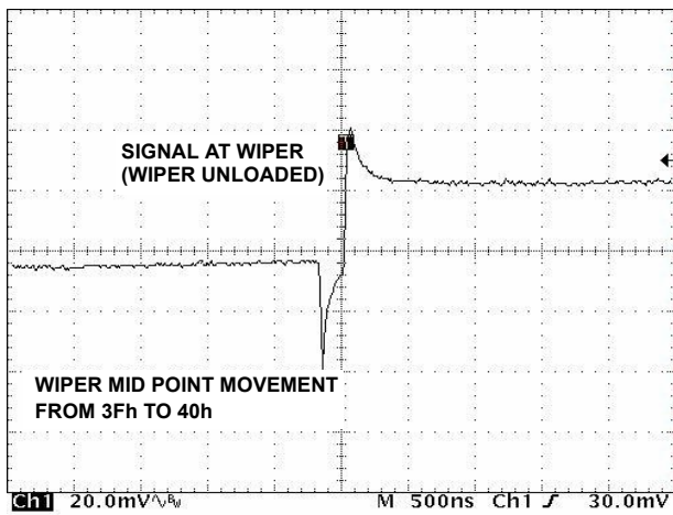
FIGURE 13. MIDSACLE GLITCH, CODE 3Fh TO 00h
