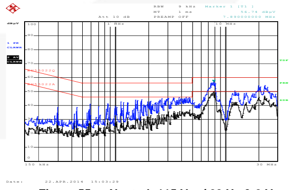
Figure 55. Neutral: 115 V AC / 60 Hz & 9 V O
