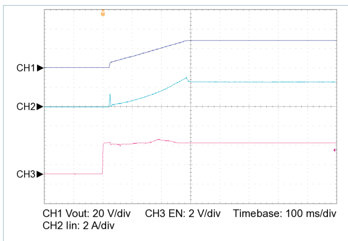
Figure 17 — Startup from EN, V_{IN} = 100\text{ V} , C_{OUT\_EXT} = 20000\text{ μF} , R_{LOAD} = 3.256\text{ Ω}
