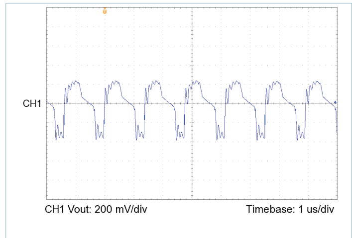
Figure 19 — Output voltage ripple, V_{IN} = 100\text{ V} , V_{OUT} = 28.0\text{ V} , C_{OUT\_EXT} = 1000\text{ μF} , R_{LOAD} = 3.256\text{ Ω}
