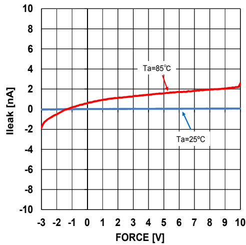
[SW] FORCE Leakage Current
