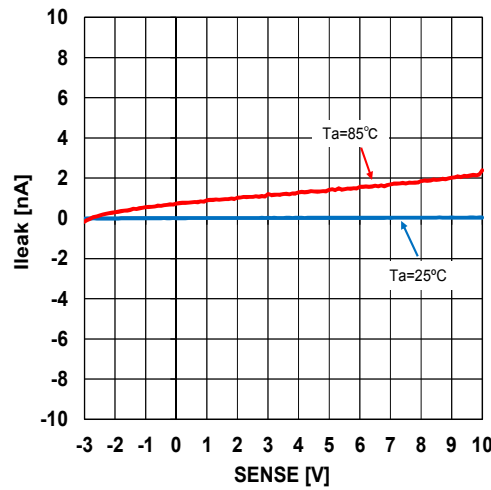
[SW] SENSE Leakage Current
