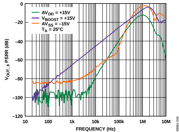
Figure 30. V_{OUT\_x} PSRR vs. Frequency
