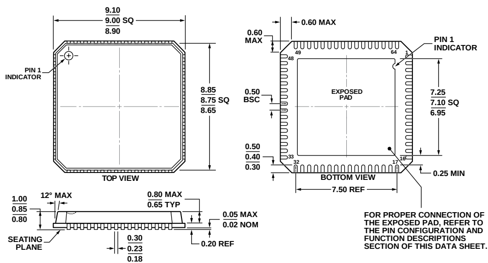
Figure 86. 64-Lead Lead Frame Chip Scale Package [LFCSP_VQ] 9 mm x 9 mm Body, Very Thin Quad (CP-64-3) Dimensions shown in millimeters
