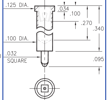
4582-0-15-XX-23-XX-10-0 Square press-fit in .040 plated thru hole
