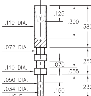
8067-0-19-XX-13-XX-10-0 Wire Crimp Termination. Accepts wire sizes 24 AWG Max. / 28 AWG Min.
