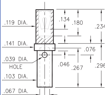
0368-0-33-XX-13-XX-10-0 Wire Crimp Termination. Accepts wire sizes 16 AWG Max. / 20 AWG Min.
