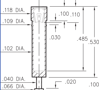
0496-0-15-XX-23-XX-10-0 Press-fit in .106 mounting hole
