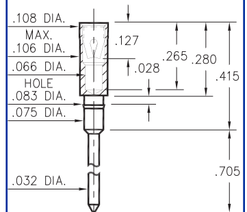
1105-0-15-XX-13-XX-04-0 Press-fit in .080 mounting hole
