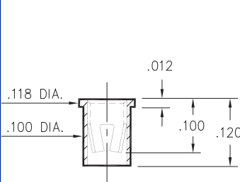
9372-0-15-XX-23-XX-10-0 Solder mount in .102 min. mounting hole
