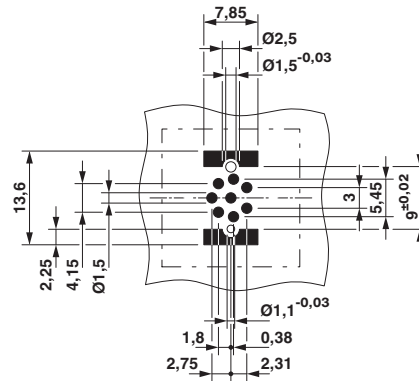
Drilling diagram
