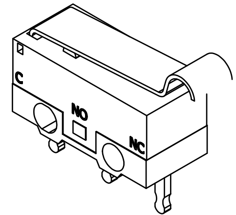
ISOMETRIC
