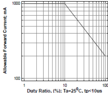
Allowable Forward Current Vs Duty Ratio
