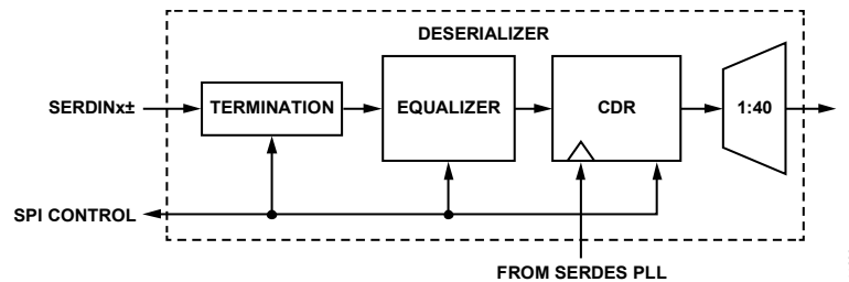
Figure 42. Deserializer Block Diagram
