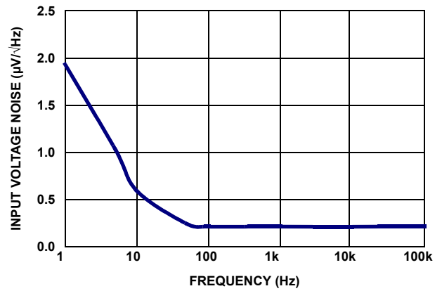
FIGURE 12. EL8173 VOLTAGE NOISE DENSITY
