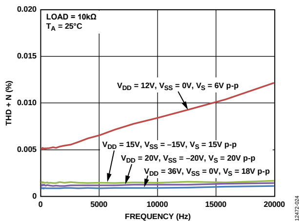
Figure 25. THD + N vs. Frequency, \pm 15\text{V} Dual Supply
