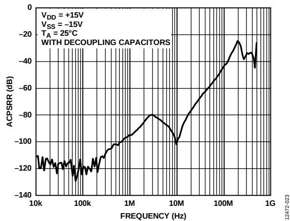
Figure 24. ACPSRR vs. Frequency, \pm 15\text{V} Dual Supply
