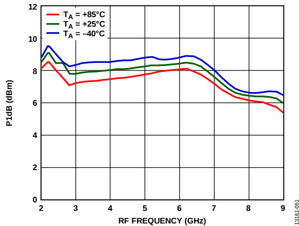
Figure 55. Input P1dB vs. RF Frequency at Various Temperatures, LO Drive = 15 dBm
