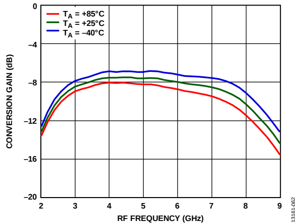
Figure 68. Conversion Gain vs. RF Frequency at Various Temperatures, LO Drive = 15 dBm
