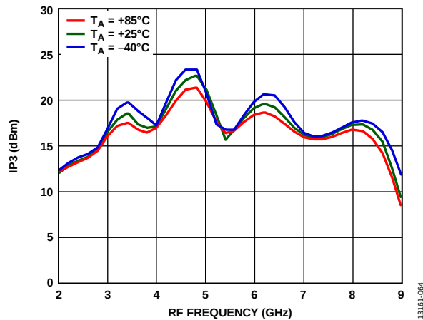
Figure 69. Input IP3 vs. RF Frequency at Various Temperatures, LO Drive = 15 dBm
